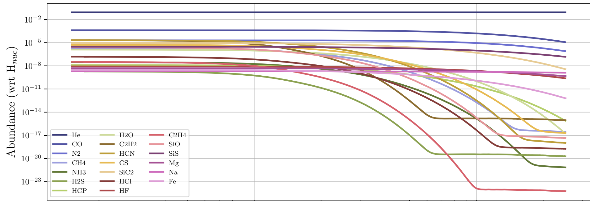
Particle 91127 - Daughter Molecules
