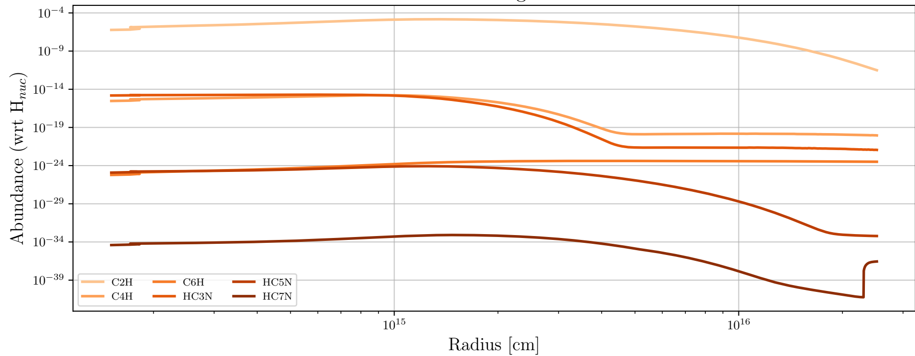
Particle 91127 - Daughter Molecules
